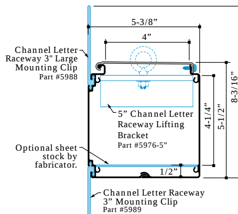
2 Piece 5" Channel Letter Raceway w/Raceway Cover Part #1971 & 1972 Part#1976
