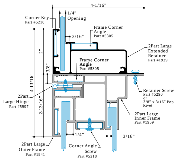
2Part Large Extended Retainer Part #1939 2Part Large Vandal System Parts #1959 and Part #1941
