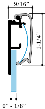
Snap Frame Part #1899 Snap Frame Flat Cover Part #1895
