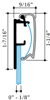
Snap Frame Part #1899 Snap Frame Flat Cover Part #1895
