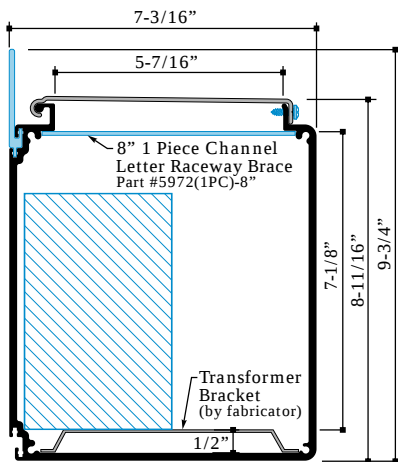
1 Piece 8" Channel Letter Raceway w/Raceway Cover Part #1980 Part#1986
