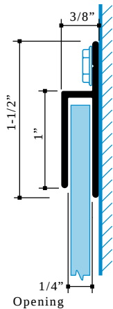
1" H-Molding Part #1945
