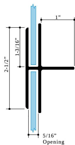
2-1/2" Divider Part #1920
