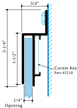
1.5" Z-Molding Part #1947
