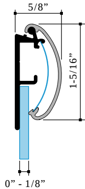
Snap Frame Part #1899 Snap Frame Radius Cover Part #1896
