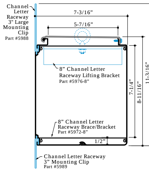
2 Piece 8" Channel Letter Raceway w/Raceway Cover Part #1981 & 1982 Part #1986
