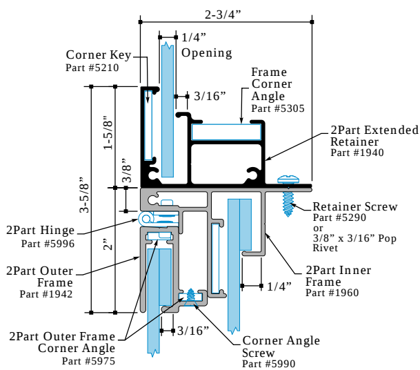
2Part Extended Retainer Part #1940 2Part Vandal System Parts #1960 and Part #1942
