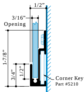
3/4" Wall Frame Part #1948
