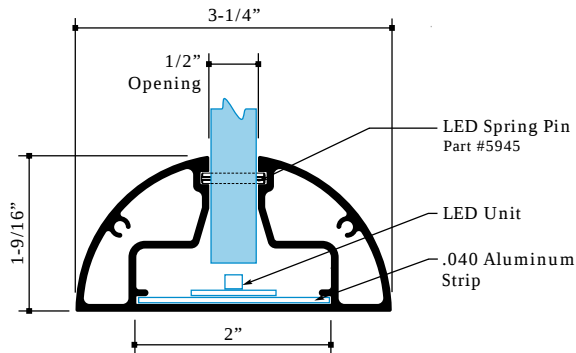
Edge Lit LED 1/2 Round Part #1995
