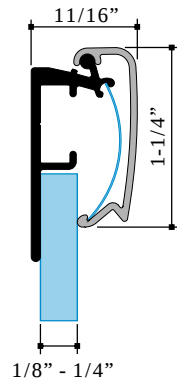
Large Snap Frame Part #1898 Snap Frame Flat Cover Part #1895
