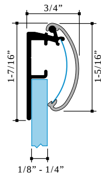
Large Snap Frame Part #1898 Snap Frame Radius Cover Part #1896
