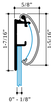
Snap Frame Part #1899 Snap Frame Radius Cover Part #1896
