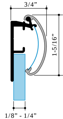
Large Snap Frame Part #1898 Snap Frame Radius Cover Part #1896
