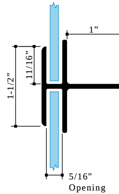
1-1/2" Divider Part #1910
