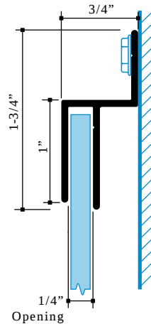
1" Z-Molding Part #1946
