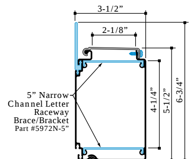
2 Piece 5" Narrow Channel Letter Raceway w/Raceway Cover Part #1971 & 1972N Part#1976N
