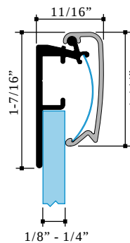
Large Snap Frame Part #1898 Snap Frame Flat Cover Part #1895
