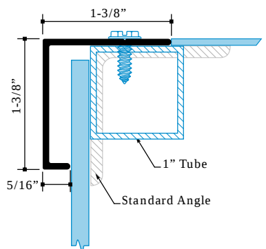
1-3/8" L-Molding Part #1943
