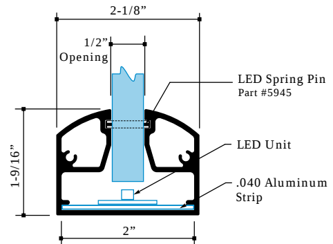
Edge Lit LED 1/4 Round Part #1996
