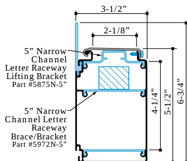
1 Piece 5" Narrow Channel Letter Raceway w/Raceway Cover Part #1970N Part#1976N
