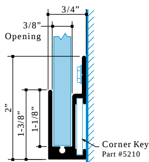
1-3/8" Wall Frame Part #1949
