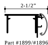
Part #1899/#1896
