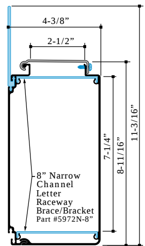
2 Piece 8" Narrow Channel Letter Raceway w/Raceway Cover Part #1981 & 1982N Part#1986N
