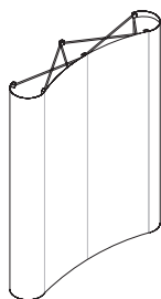
6' full height slim-line display system footprint dimensions: 87.56"h x 73"w x 19.25"d
