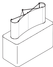
6' tabletop footprint dimensions: 30.625"h x 73"w x 19.25"d
