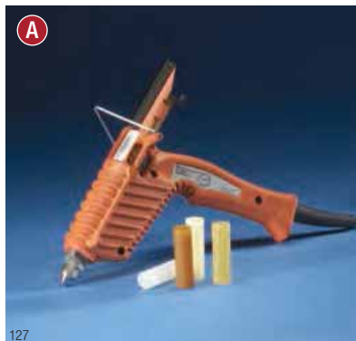
3M™ Hot Melt Applicator LT. Low-medium volume using low melt adhesive. UPC# 021200-82245
