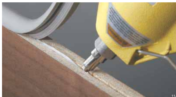
Bond extruded plastic edge molding to particle board core.
