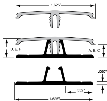
"H" Extrusion
