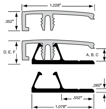
"J" Extrusion
