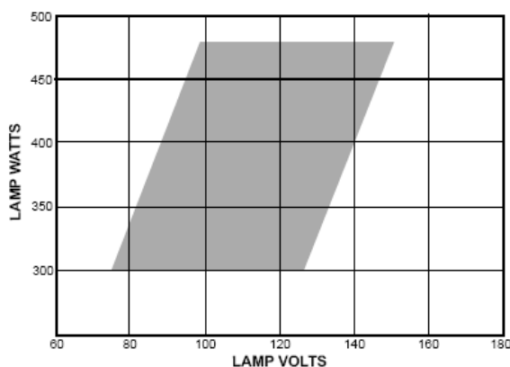
TRAPEZOID – 400W HPS, 100V Lamp
