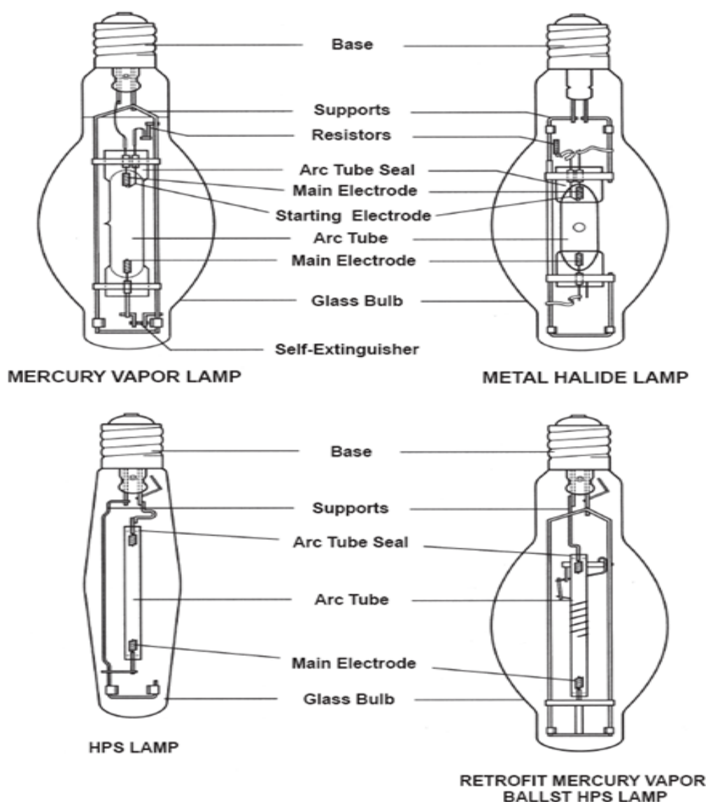
Figure1. Components of HID lamp designs.
