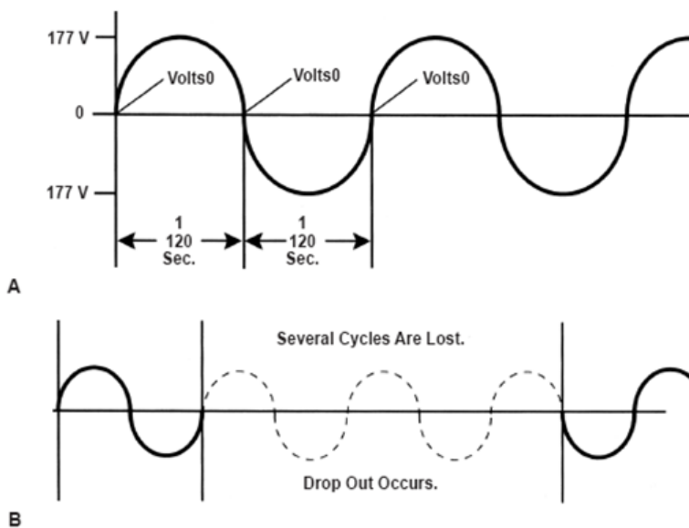
Figure 15. (A) Voltage actually is cut to the lamp every time alternating current changes direction. This happens 120 times per second with 60 Hertz AC power. (B) When several cycles of AC current drop out or are lost, the lamp will turn OFF
