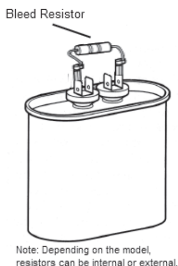
Figure17. A missing or defective capacitor resistor can cause a no-start problem.
