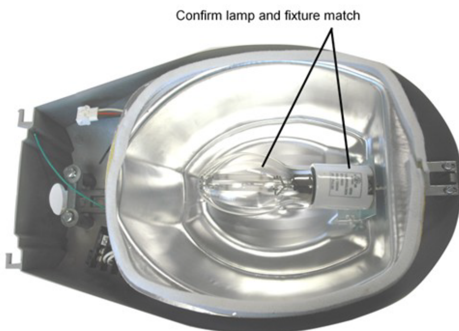
Figure14. Checking the correct lamp.
